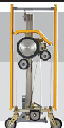
Kleinseilsäge small wire saw WB6P
